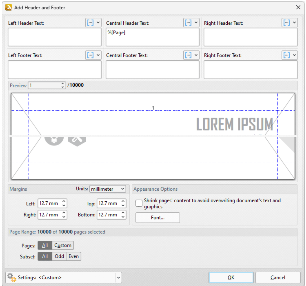
Figure 4. %[Page] Macro Output Example, Three Page Document
