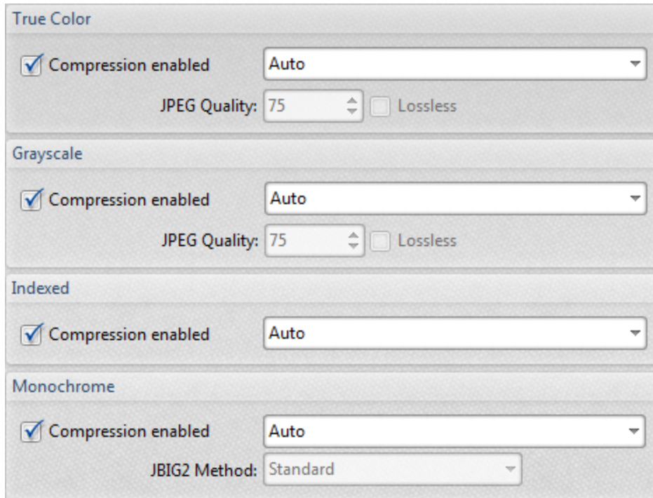
Figure 9. Image Post-Processing Options Dialog Box
