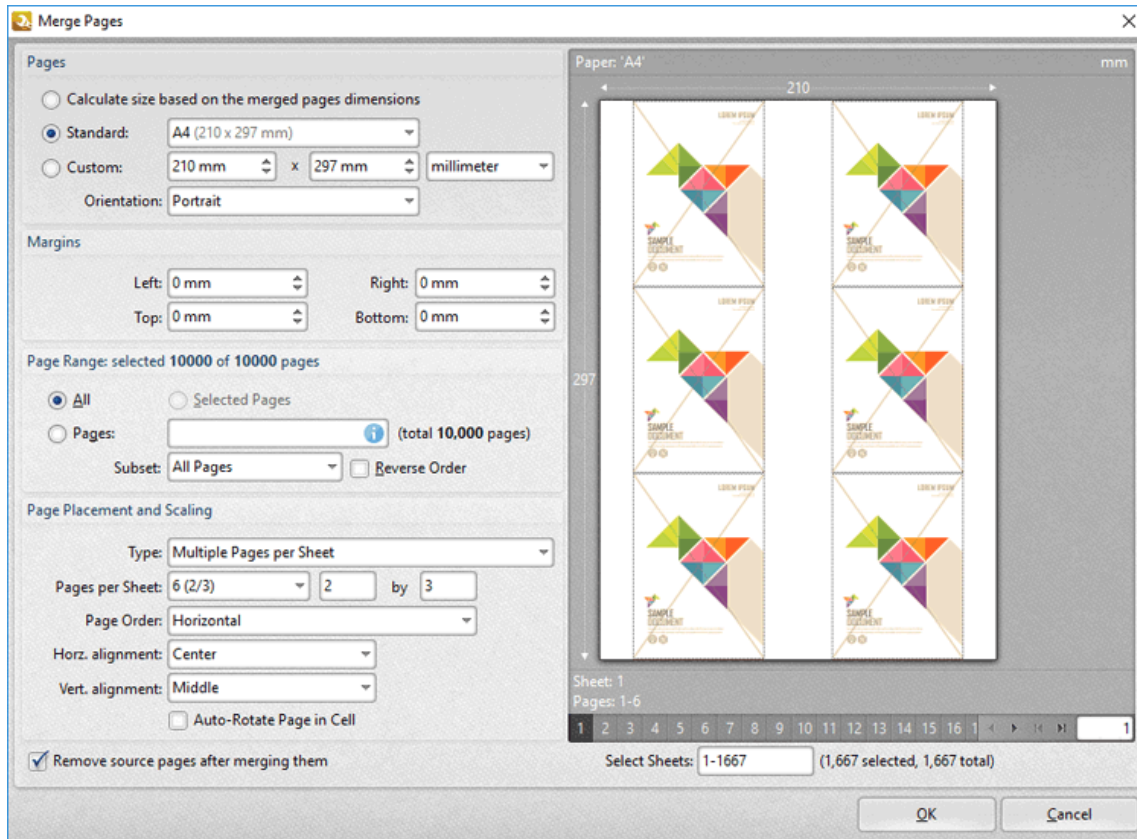
Figure 2. Merge Pages Dialog Box
