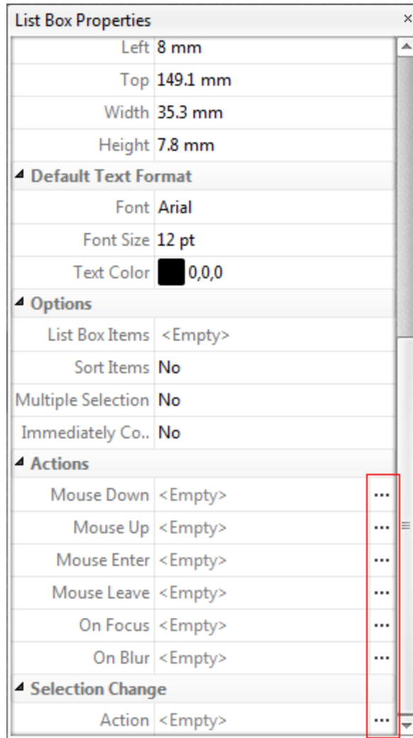
Figure 7. List Box Properties Pane, Action Ellipses
