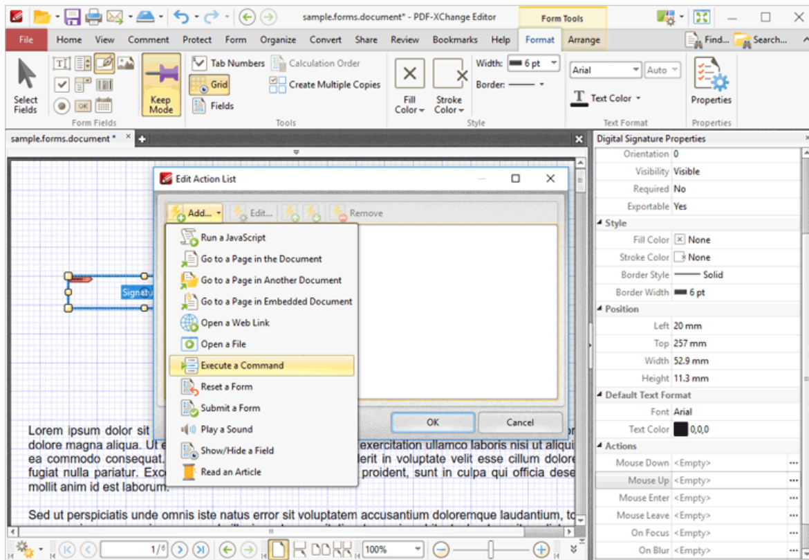
Figure 14. Edit Action Dialog Box, Execute a Command
